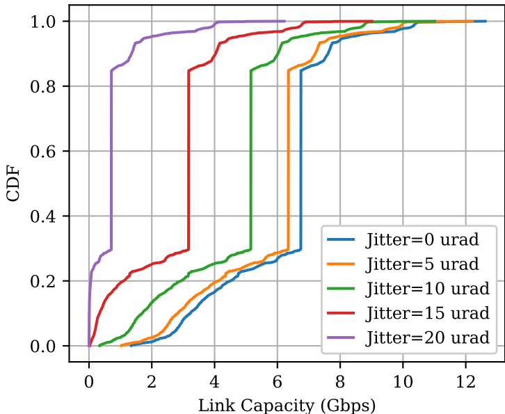
Link Capacities in Regular Walker-Delta Constellation
