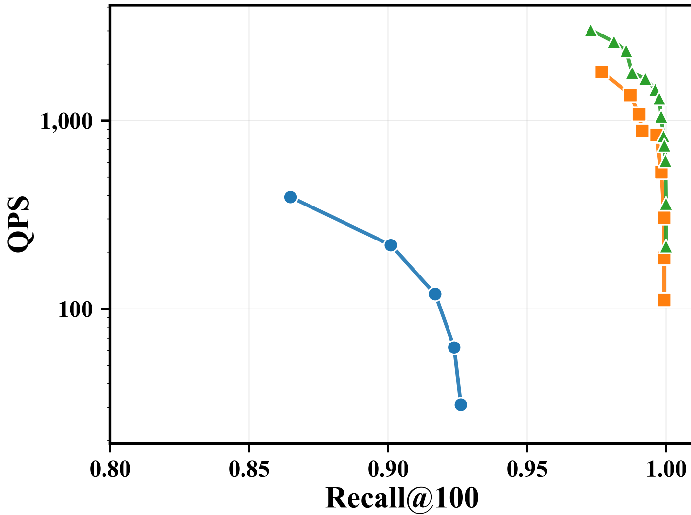
CC-News original
