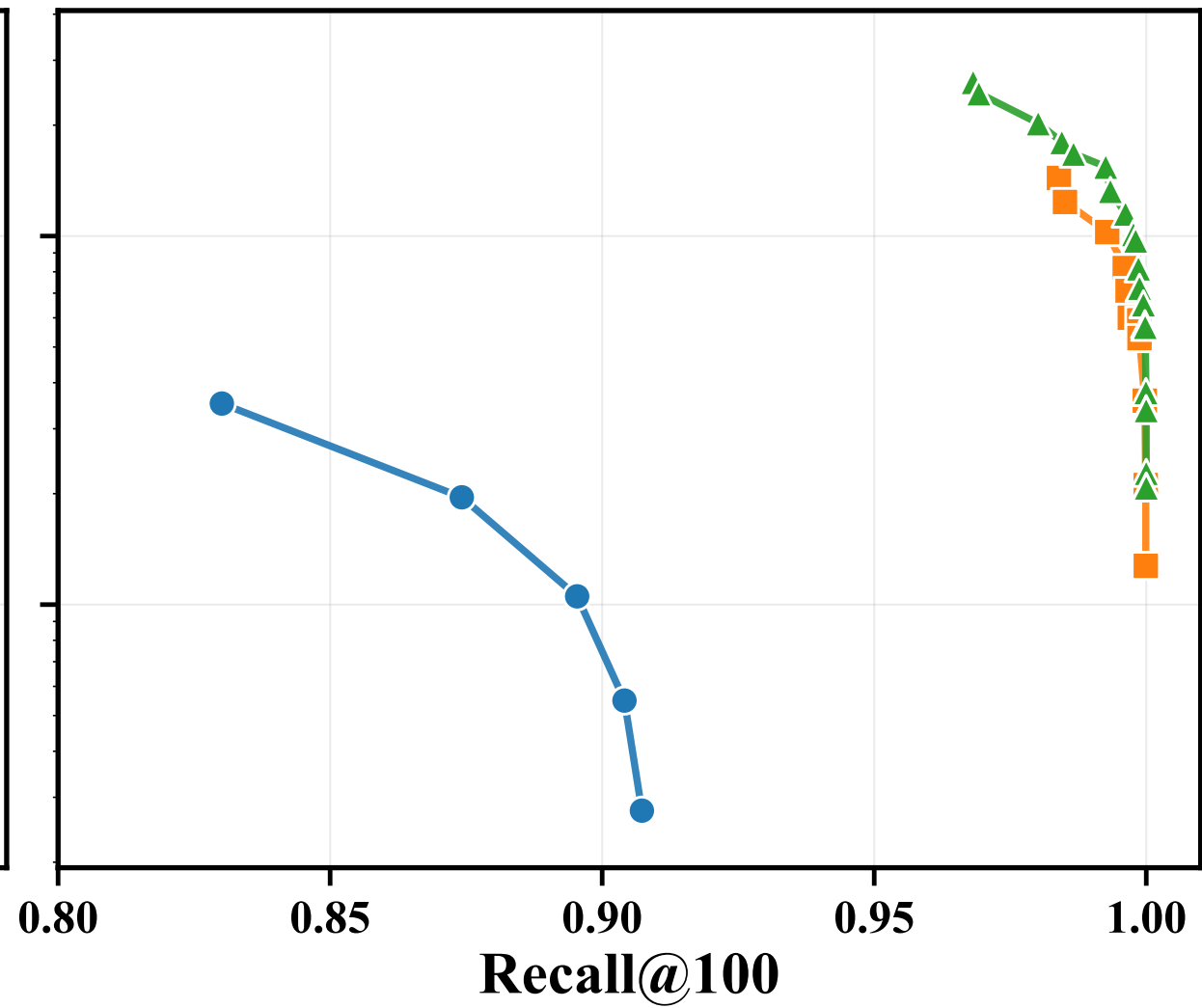
CC-News shuffled
