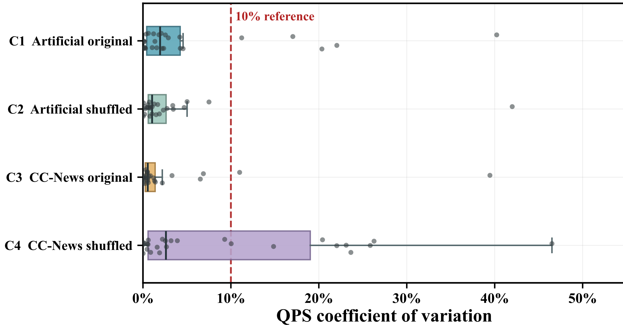
QPS variation across correlation workloads
