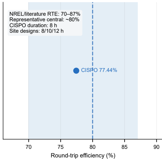
Pumped hydro: technical assumptions
