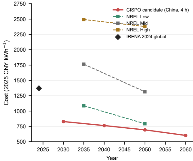
Battery: energy-equivalent cost
