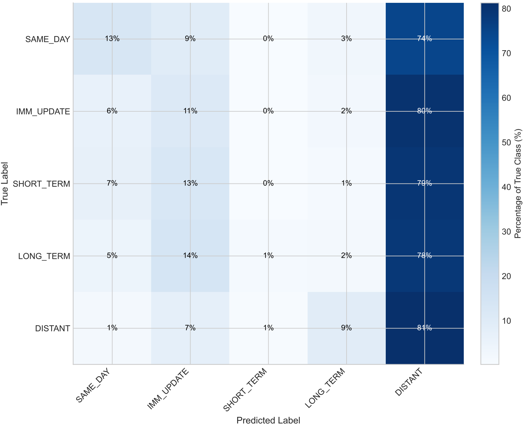
Confusion Matrix: Temporal Threading (Stage 3)
