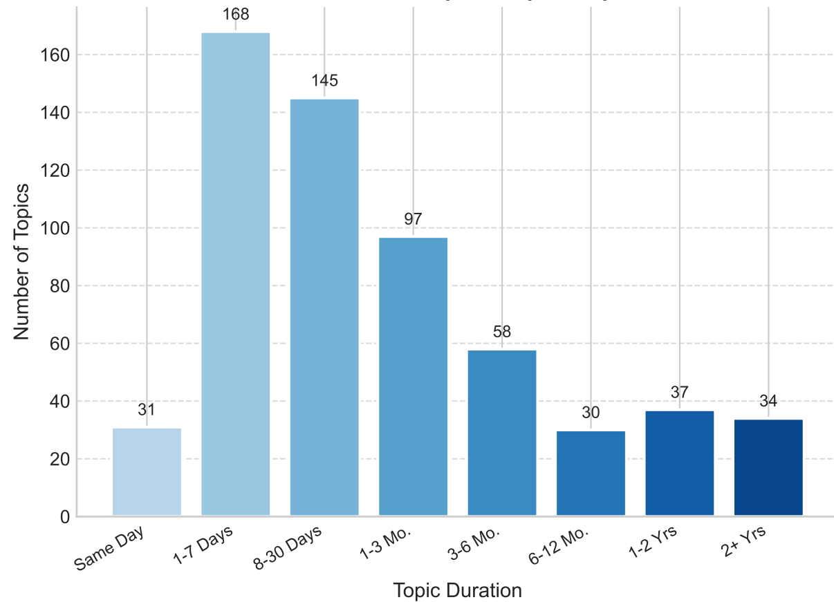
Distribution of Topic Temporal Spans
