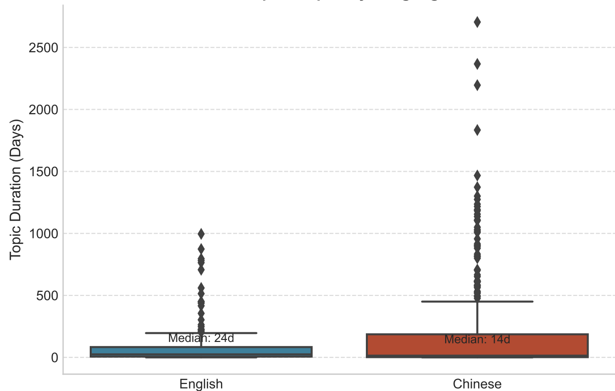
Temporal Span by Language
