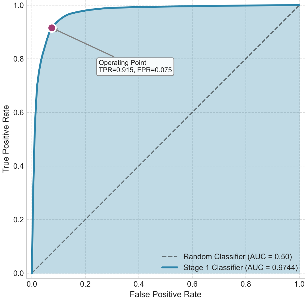
ROC Curve for Pairwise Relatedness Classification (Stage 1)
