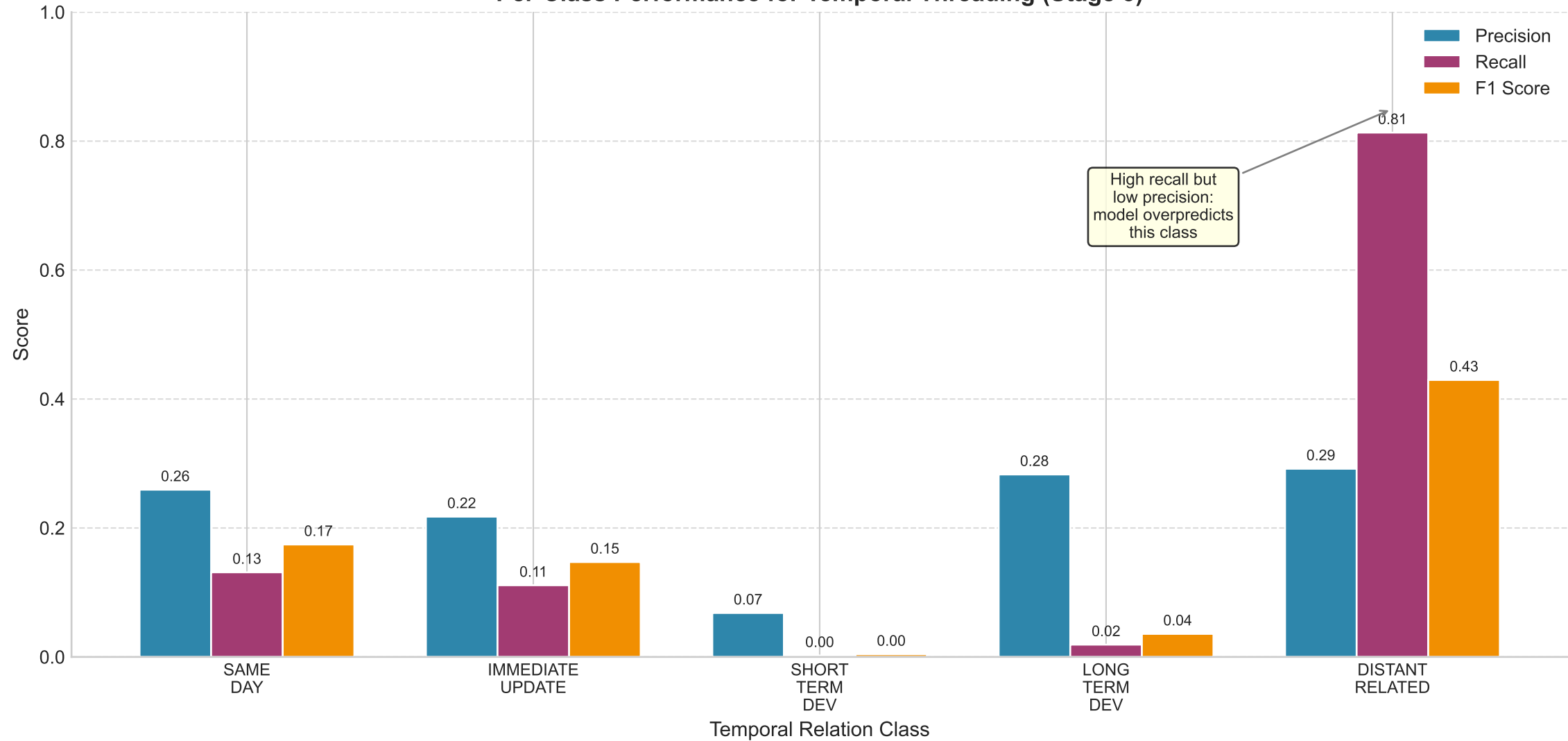
Per-Class Performance for Temporal Threading (Stage 3)
