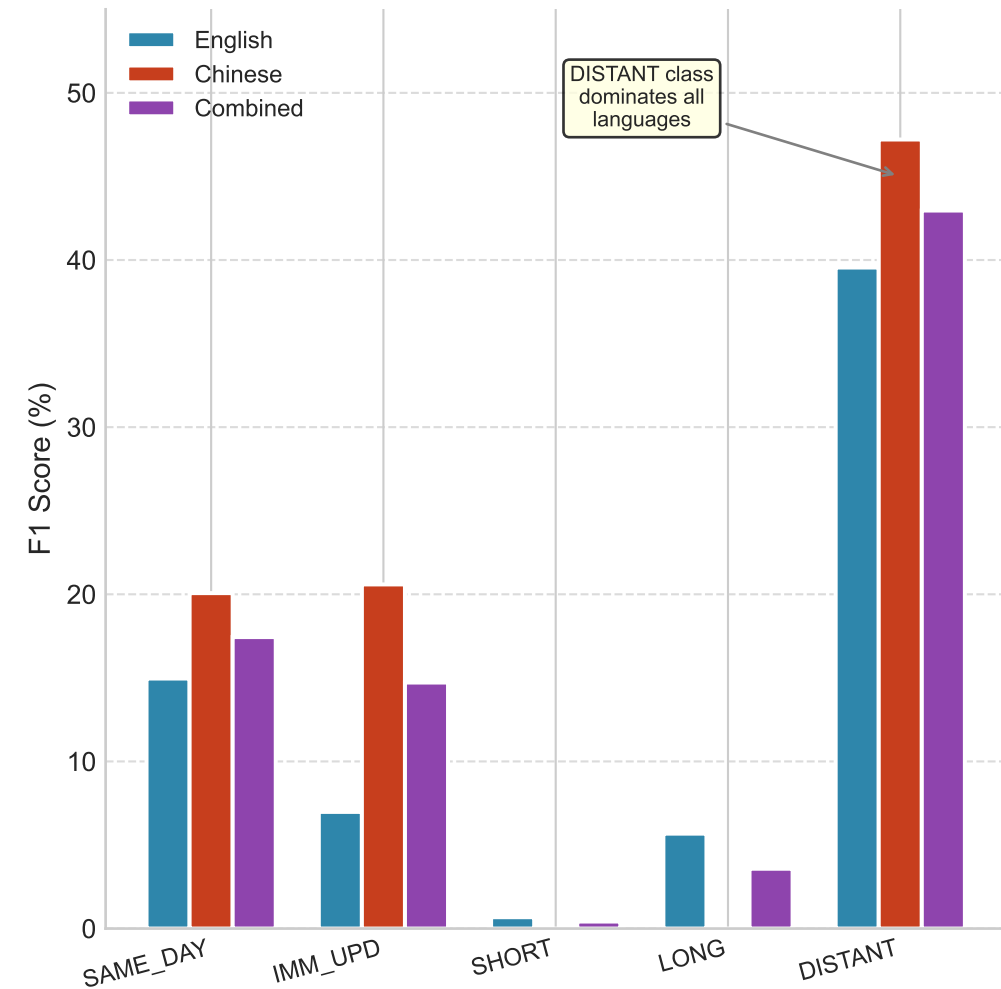
Stage 3: Per-Class F1 by Language
