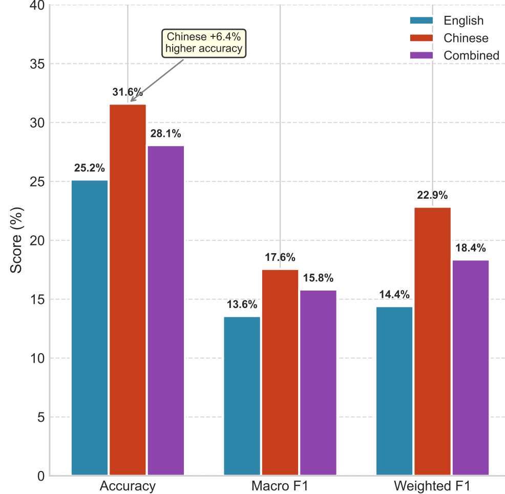
Stage 3: Per-Language Performance
