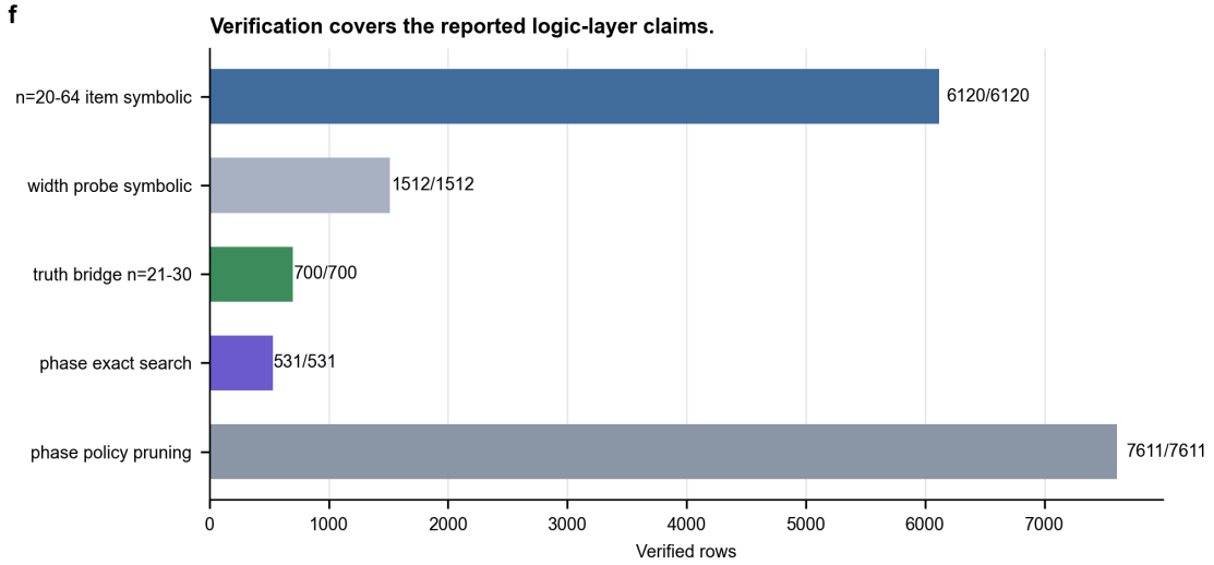
Figure 7: Verification coverage. Large term-set experiments are validated symbolically; phase-search and phase-policy rows are checked up to global phase; n = 21-30 bridge slices add complete truth table checking on selected generated functions.
