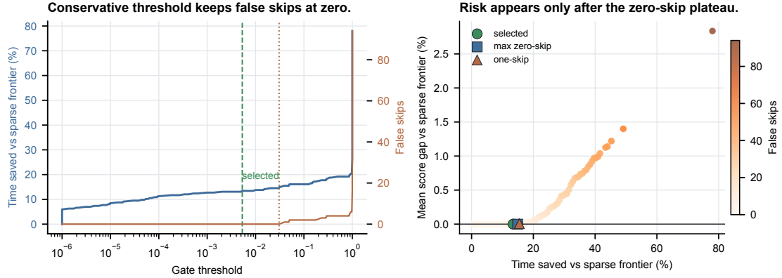
Figure 4: Sparse depth-4 gate threshold sensitivity. The sweep reuses the trained gate on the 144-pair independent-seed audit. The validation-selected threshold lies inside a zero-false-skip plateau, showing that the gate acts as a calibrated search-budget controller rather than as an ungarded depth-4 skip.
