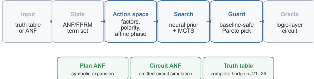
a Resource-constrained neural MCTS oracle synthesis remains verifiable at every layer.
