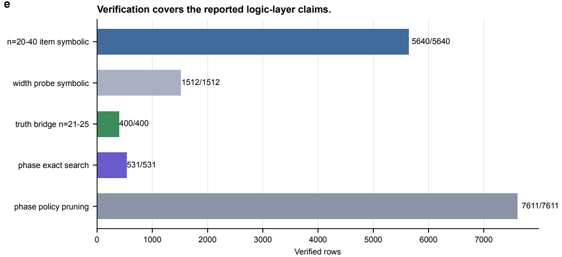
Figure 5: Verification coverage. Large term-set experiments are validated symbolically; phase-search and phase-policy rows are checked up to global phase; n = 21-25 bridge slices add complete truth table checking on selected generated functions.
