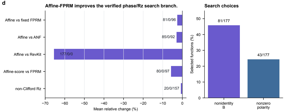
Figure 4: Affine-FPRM phase search. Affine preconditioning improves the phase-parity proxy over fixed-polarity FPRM and ANF baselines, while remaining a logical phase/Rz proxy rather than an approximate-rotation sequence.
