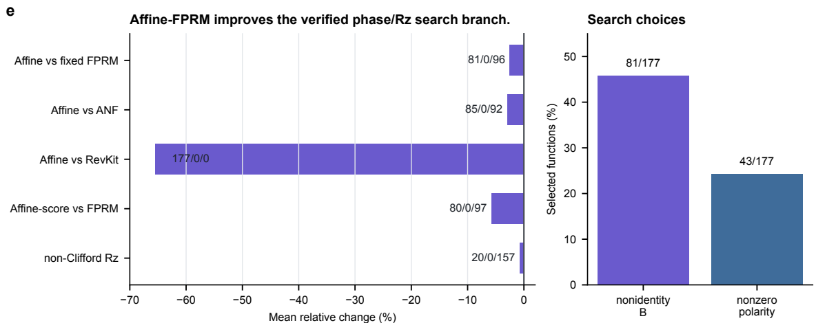
Figure 6: Affine-FPRM phase search. Affine preconditioning improves the phase-parity proxy over fixed-polarity FPRM and ANF baselines, while remaining a logical phase/Rz proxy rather than an approximate-rotation sequence.
