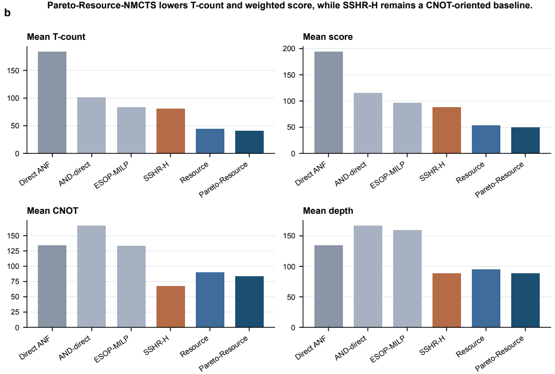
Fig. 3. Mean logical resources on the traditional slice. Pareto-Resource-NMCTS has the lowest T-count and weighted score; SSHR-H remains a strong CNOT-oriented baseline.
