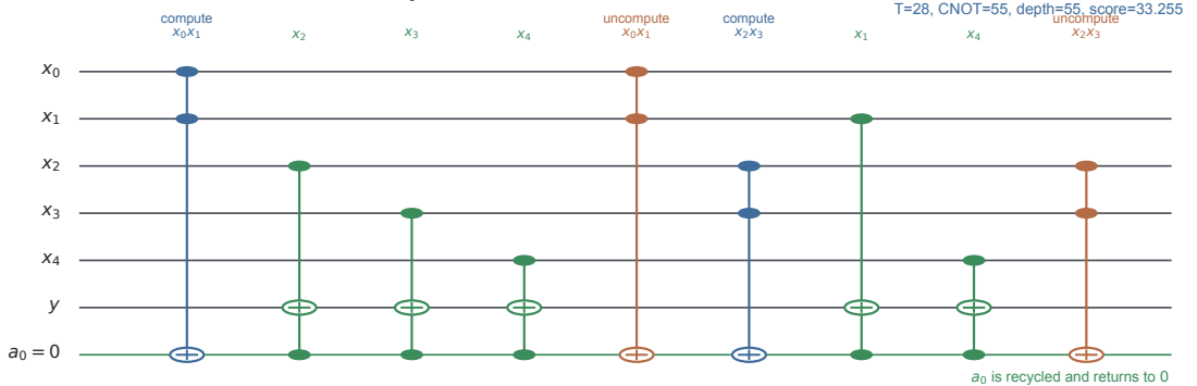
b Resource-NMCTS: two factors share one recycled line
