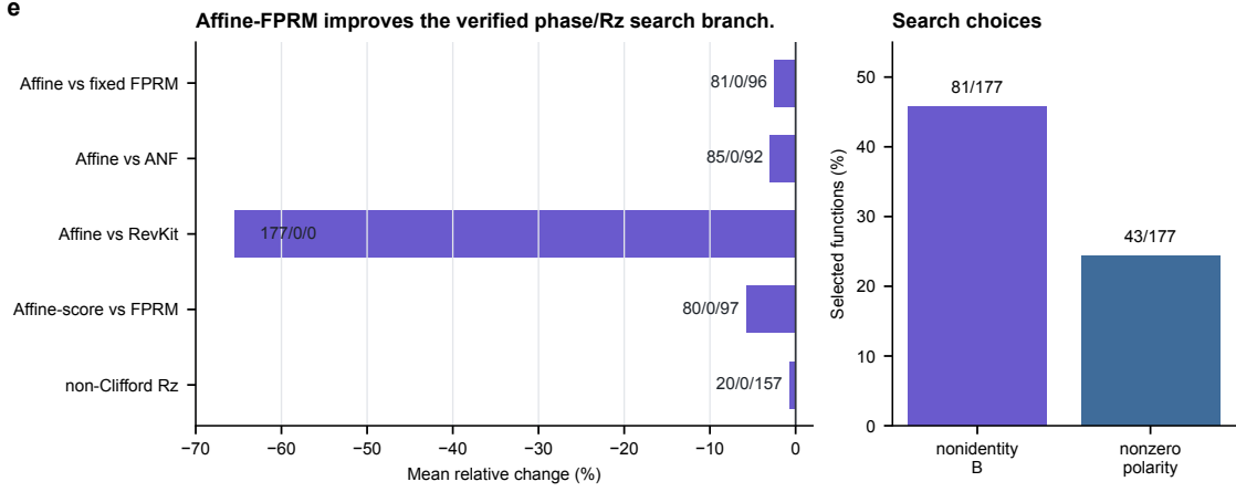
Fig. 7. Affine-FPRM phase search. Affine preconditioning improves the phase-parity proxy over fixed-polarity FPRM and ANF baselines, while remaining a logical phase/Rz proxy rather than an approximate-rotation sequence.
