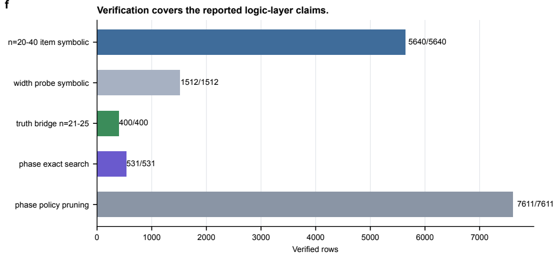
Figure 7: Verification coverage. Large term-set experiments are validated symbolically; phase-search and phase-policy rows are checked up to global phase; n = 21-25 bridge slices add complete truth table checking on selected generated functions.
