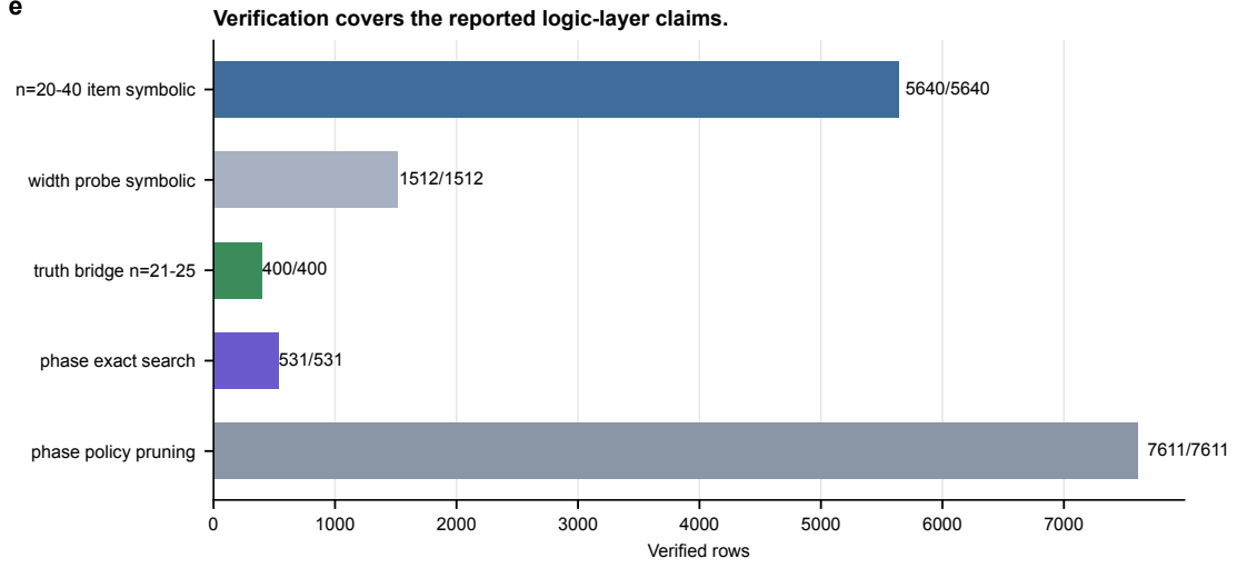
Figure 6: Verification coverage. Large term-set experiments are validated symbolically; phase-search and phase-policy rows are checked up to global phase; n = 21-25 bridge slices add complete truth table checking on selected generated functions.
