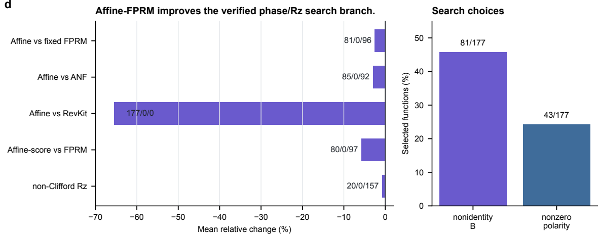
Figure 5: Affine-FPRM phase search. Affine preconditioning improves the phase-parity proxy over fixed-polarity FPRM and ANF baselines, while remaining a logical phase/Rz proxy rather than an approximate-rotation sequence.
