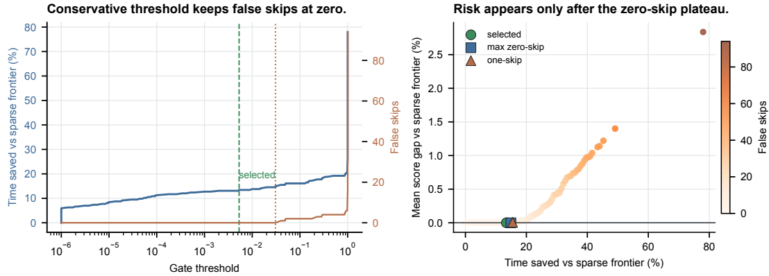
Figure 4: Sparse depth-4 gate threshold sensitivity. The sweep reuses the trained gate on the 144-pair independent-seed audit. The validation-selected threshold lies inside a zero-false-skip plateau, showing that the gate acts as a calibrated search-budget controller rather than as an ungarded depth-4 skip.
