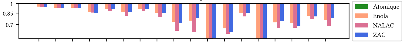
decoherence comparison
