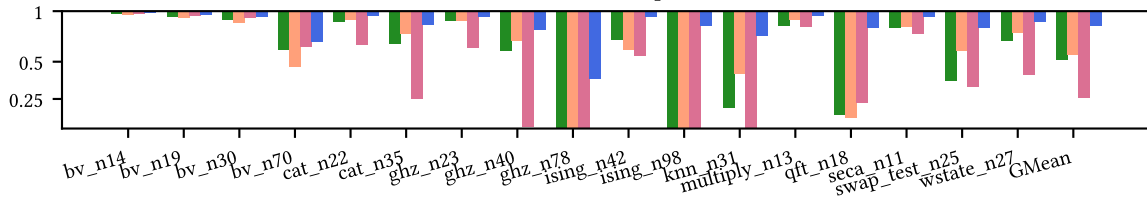
decoherence comparison
