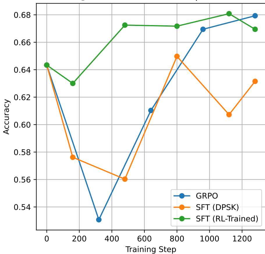
Pass@1 GSM8K Test with temperature 0
