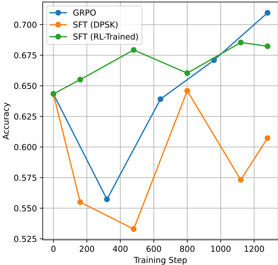
Pass@1 GSM8K Test with temperature 0.6
