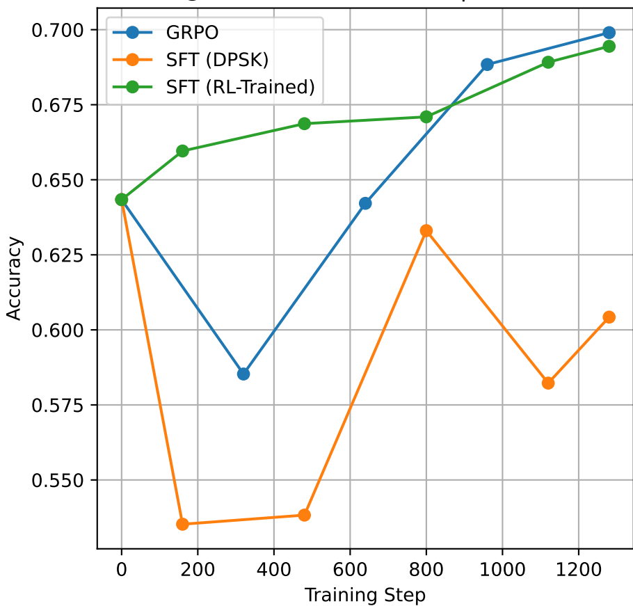
Pass@1 GSM8K Test with temperature 0.7
