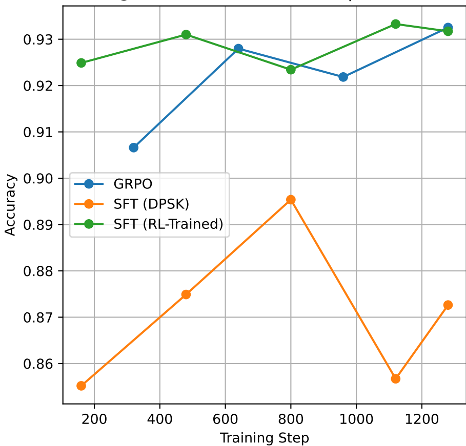
Pass@8 on GSM8K Test with Temperature 0.7
