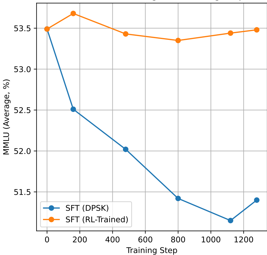
Model MMLU (Average) vs Training Step
