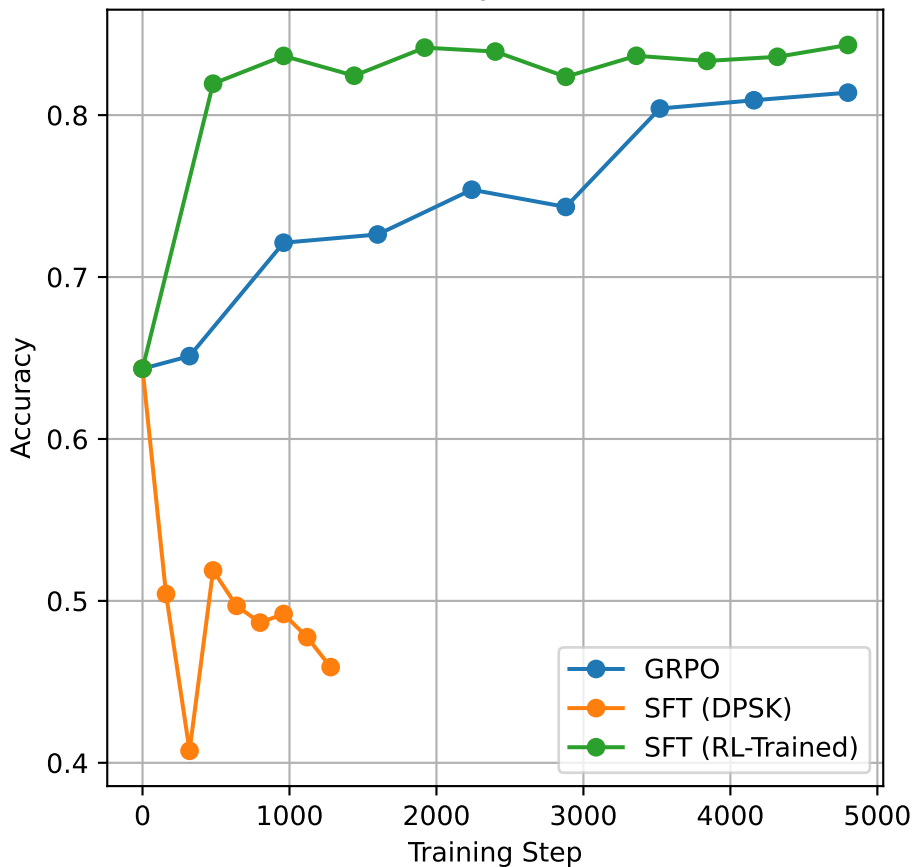
Model Accuracy on GSM8K Test
