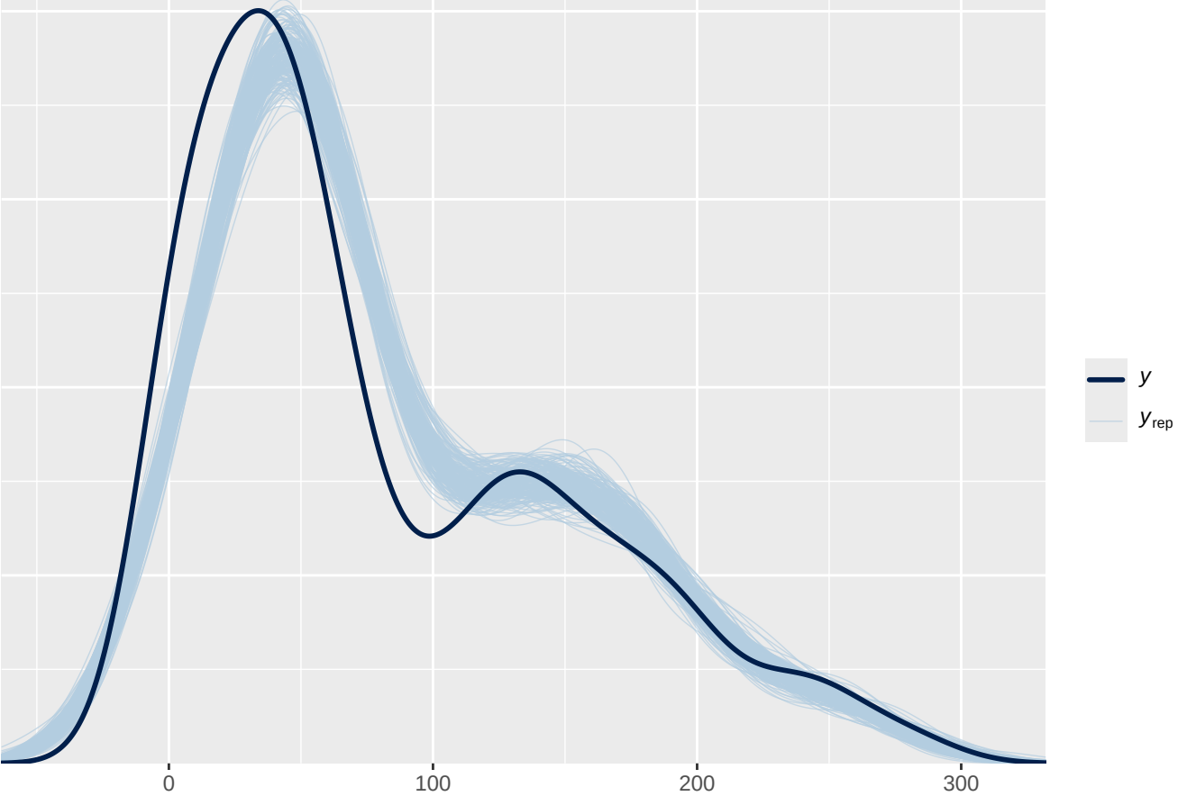
PPC density overlay: Logistic_noM
