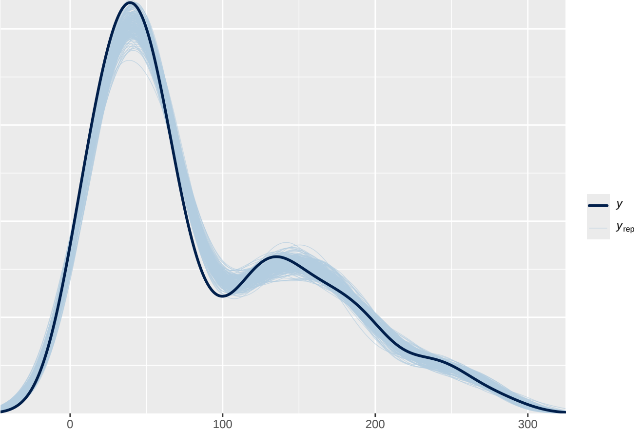
PPC density overlay: Logistic
