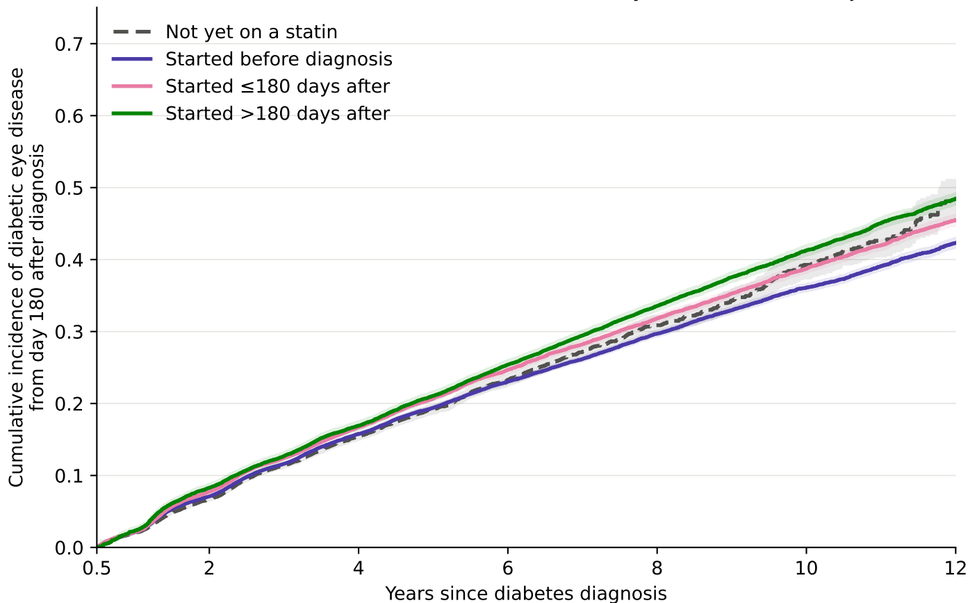
CPRD: Simon-Makuch cumulative incidence by statin state (unadjusted)
