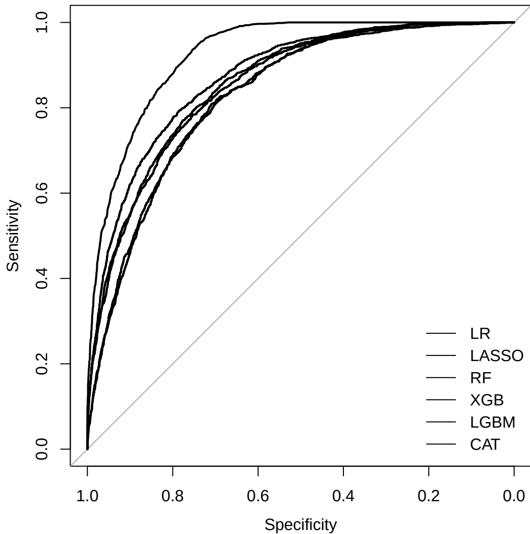
A: Training Set ROC Curves
