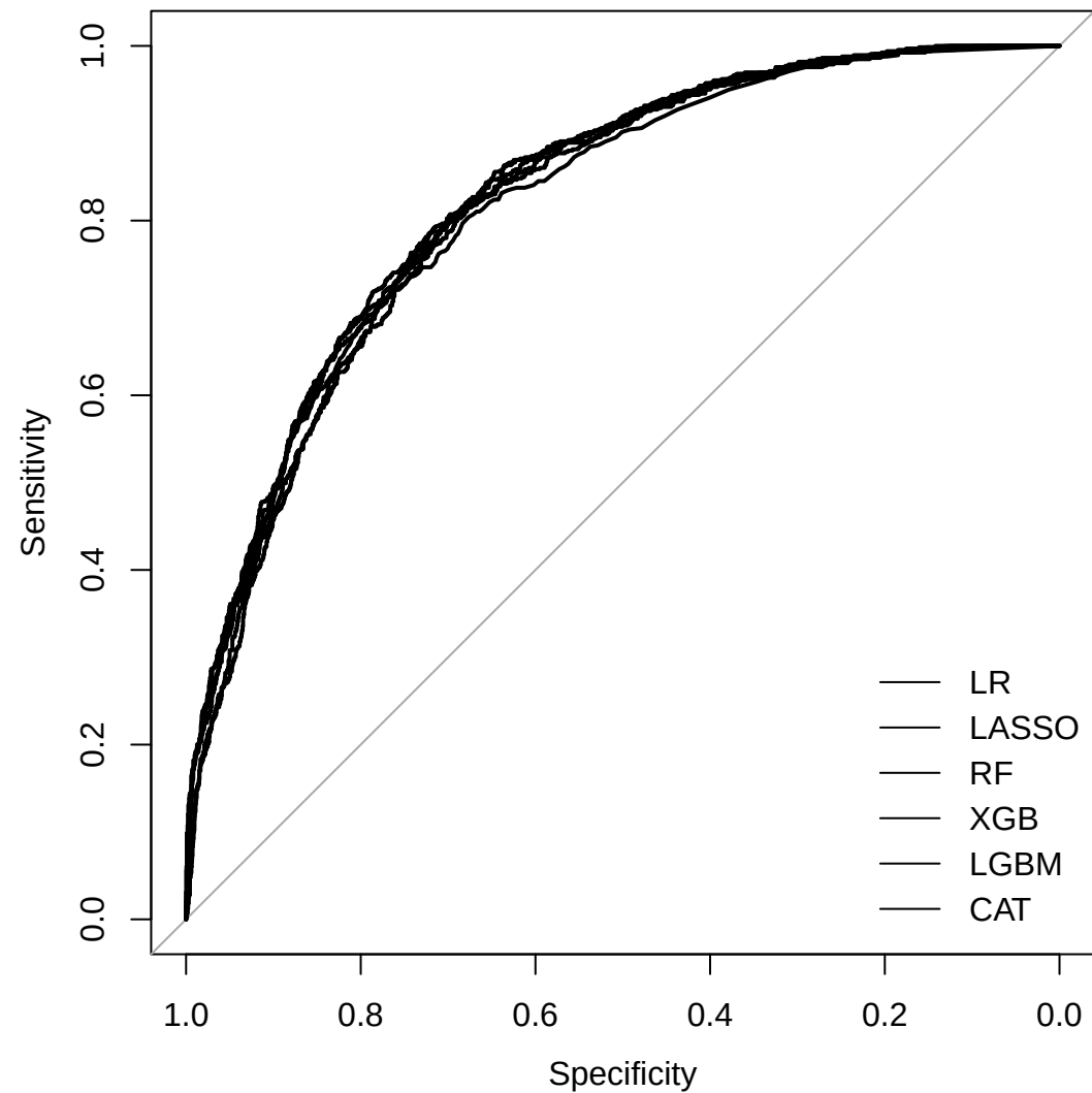
B: Testing Set ROC Curves
