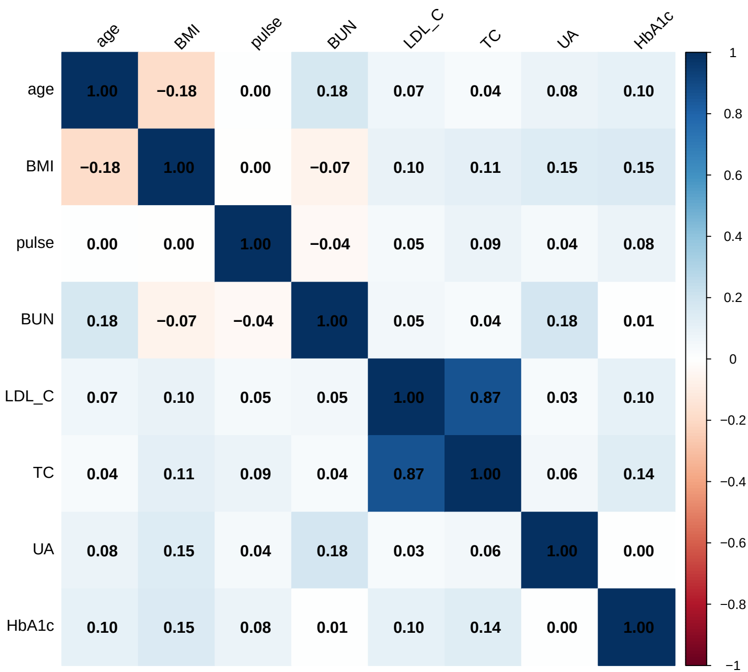
Correlation Matrix of LASSO-Selected Features
