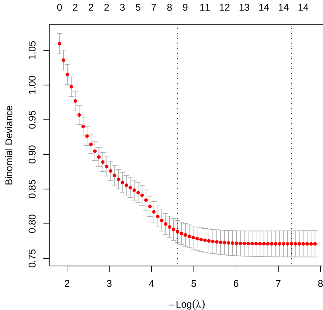
B: 10-fold Cross-validation
