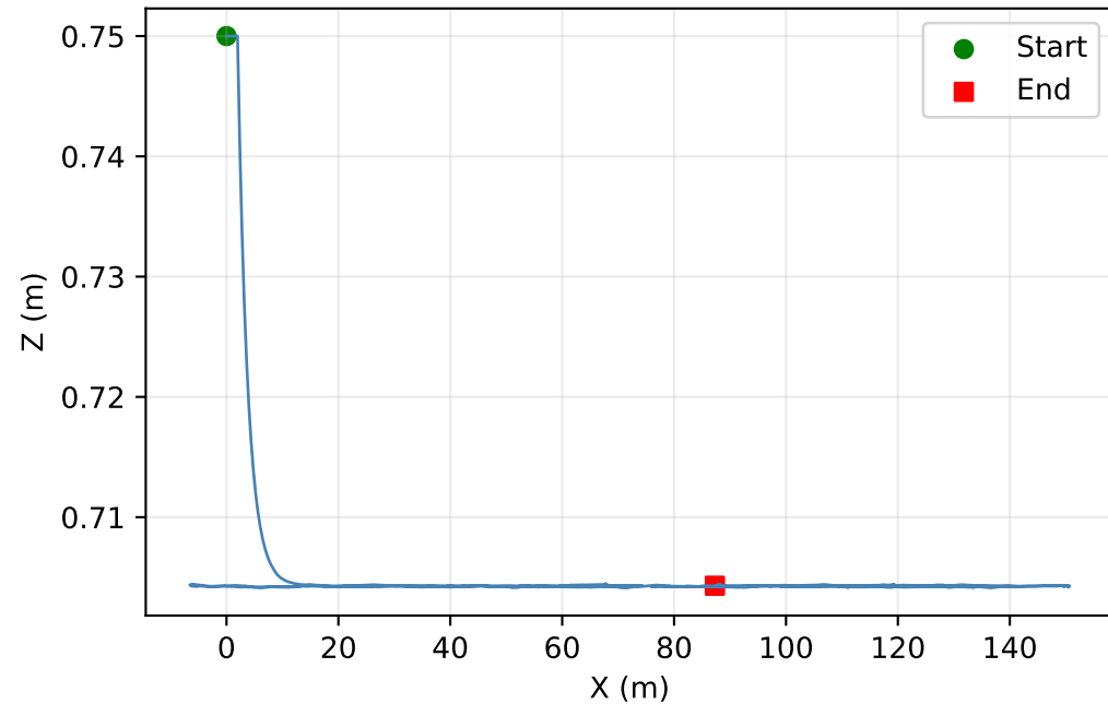
Measured travel
