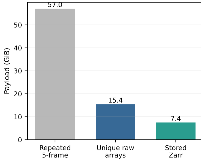
Unique-frame storage removes duplication
