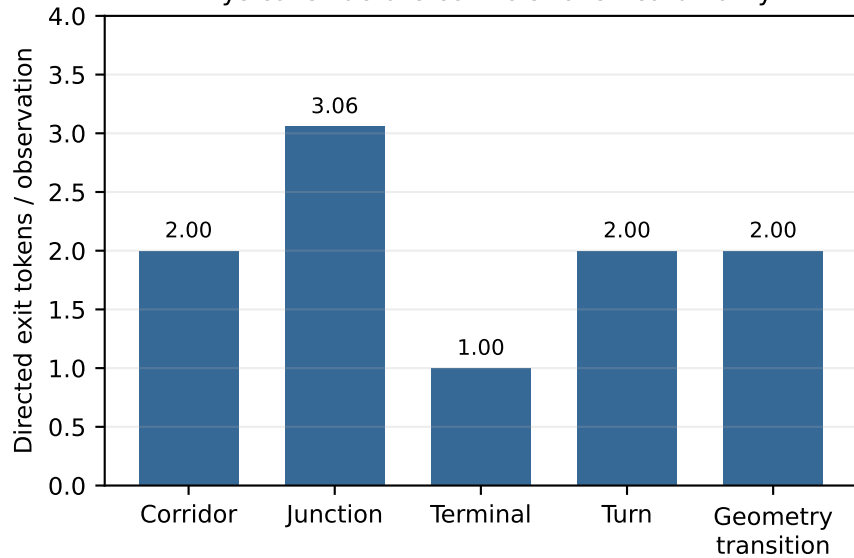
Physical structure controls token cardinality
