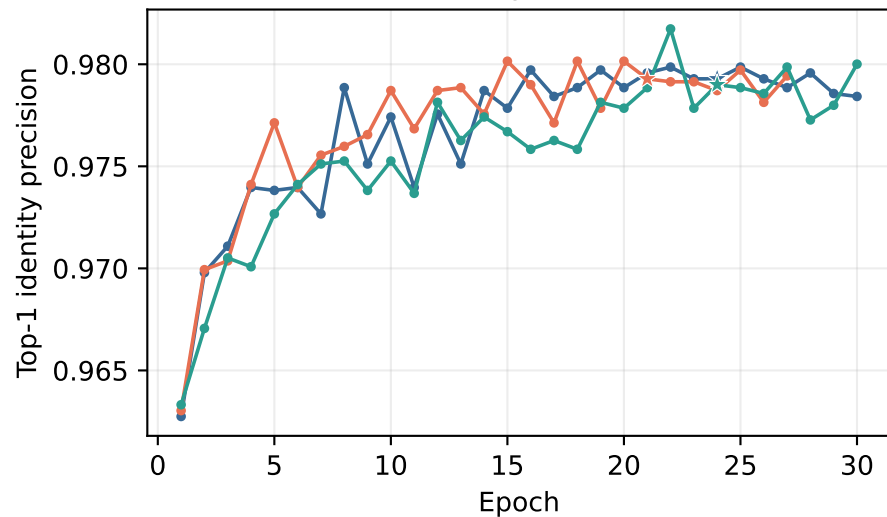
Place-descriptor retrieval
