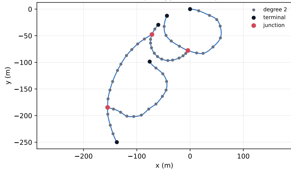
(a) Generated tunnel topology and swept axes
