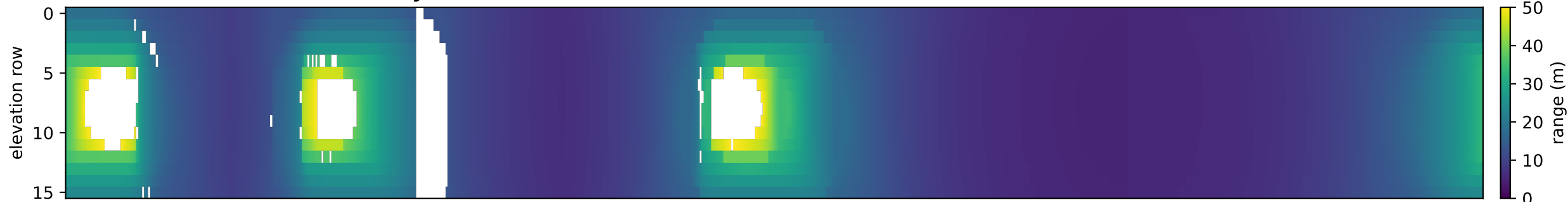
(c) Causal LiDAR frame used by the student
