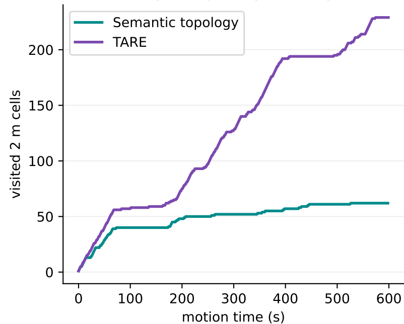
Unique trajectory coverage
