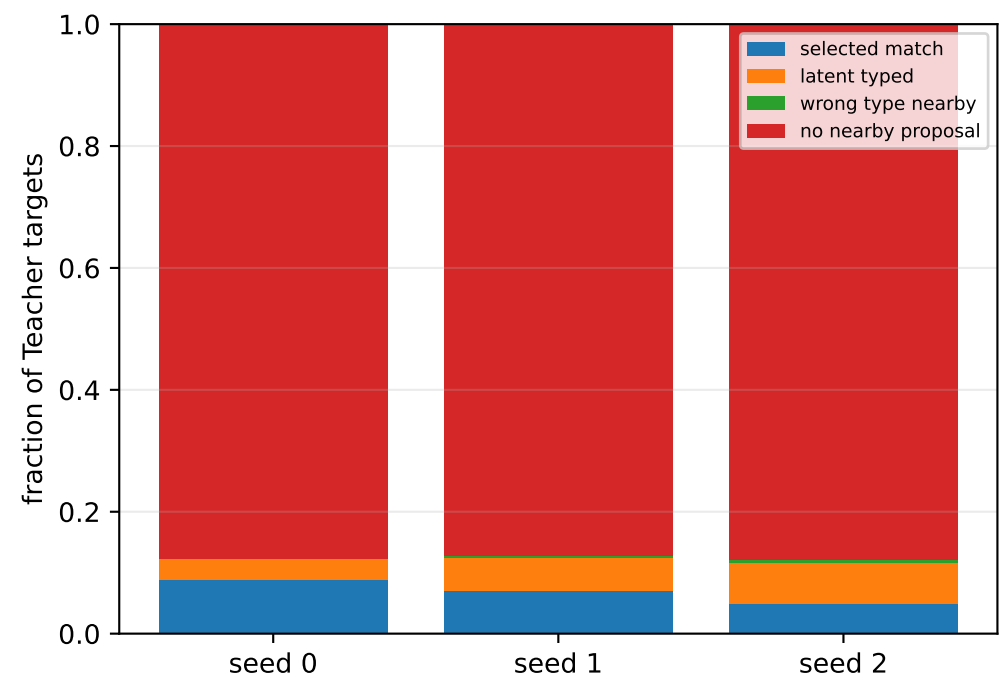
Geometry-anchored proposal attribution: free-query spatial proposal failure; exclusive F1=0.390
