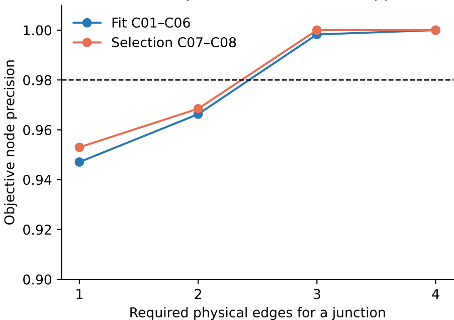
Node safety from route-diverse support
