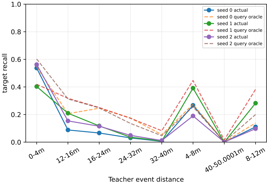
Spatial event-set failure attribution: ENCODER_SPATIAL_REPRESENTATION_INSUFFICIENT_NEW_ENCODER_OBJECTIVE_REQUIRED
