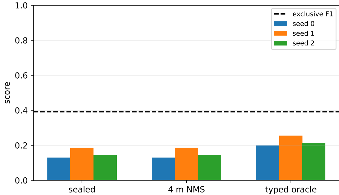
Spatial event-set failure attribution: ENCODER_SPATIAL_REPRESENTATION_INSUFFICIENT_NEW_ENCODER_OBJECTIVE_REQUIRED
