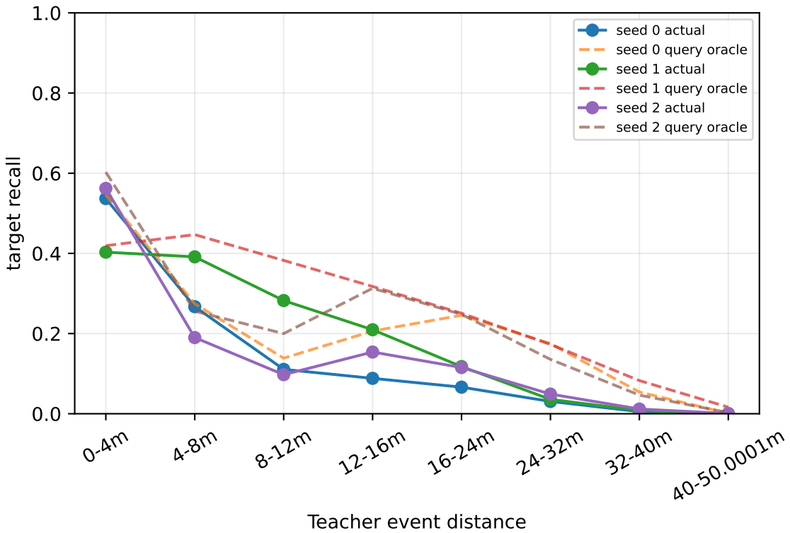
Spatial event-set failure attribution: new spatial encoder objective required
