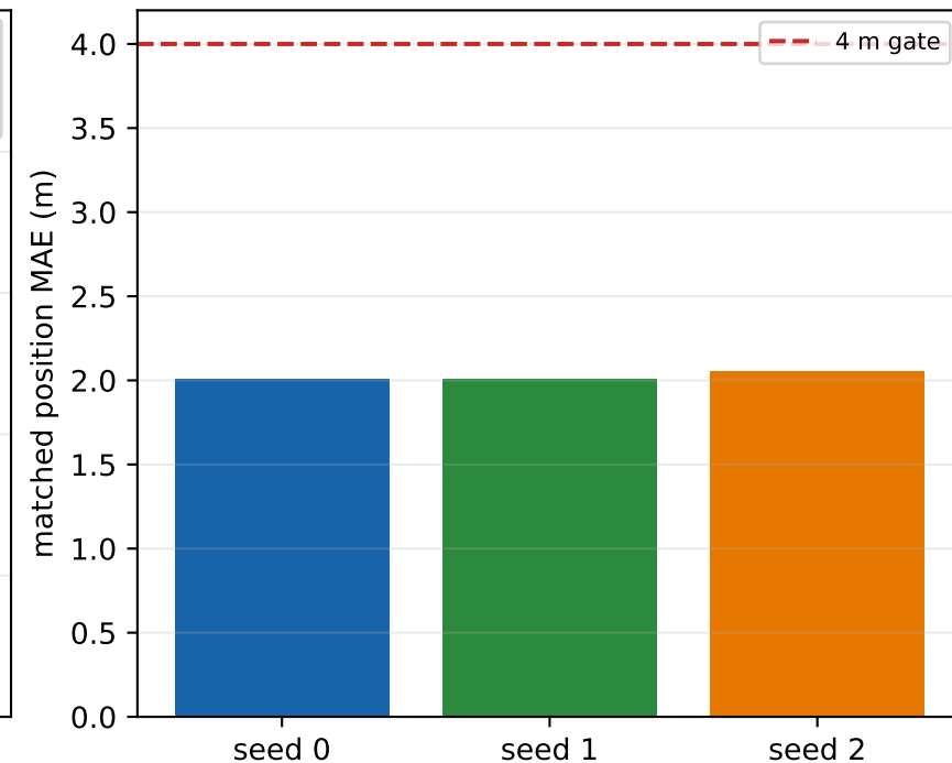
Structured localization
