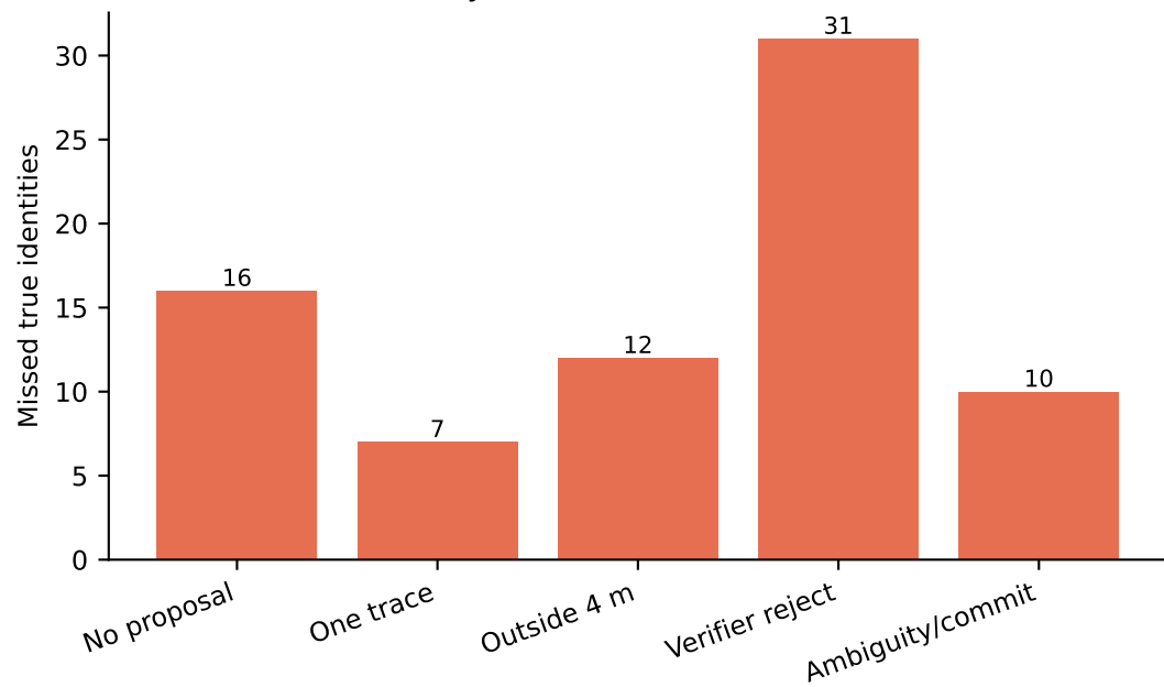
Why true nodes are still lost
