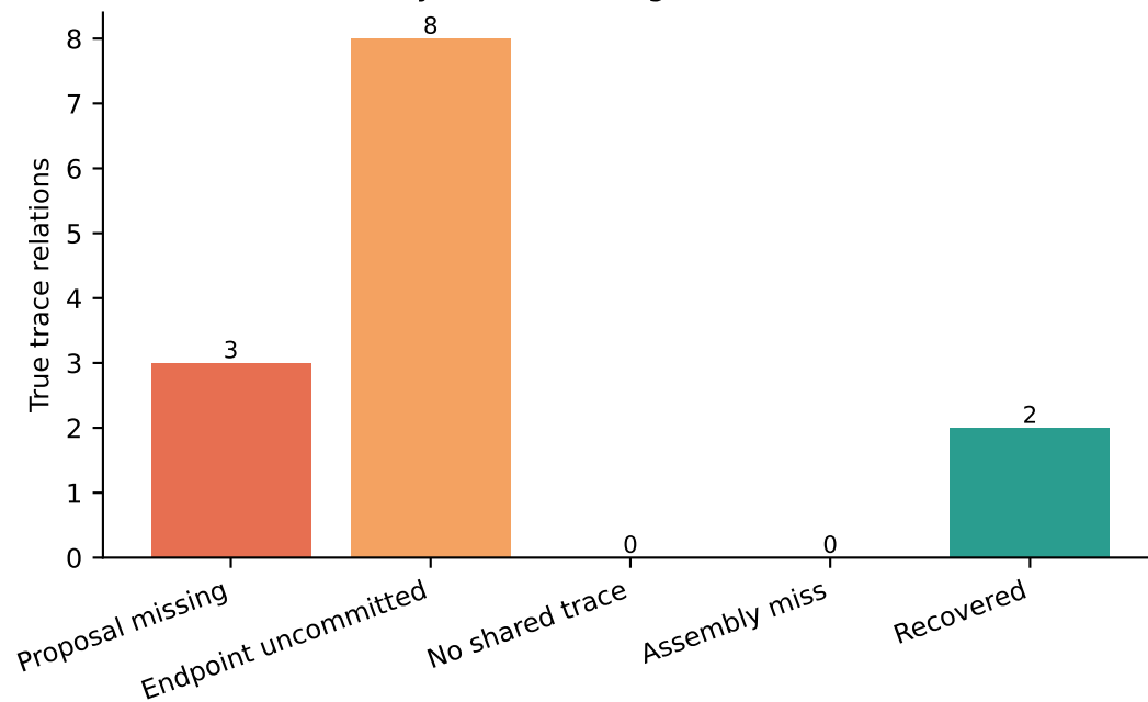
Why traversed edges are still lost
