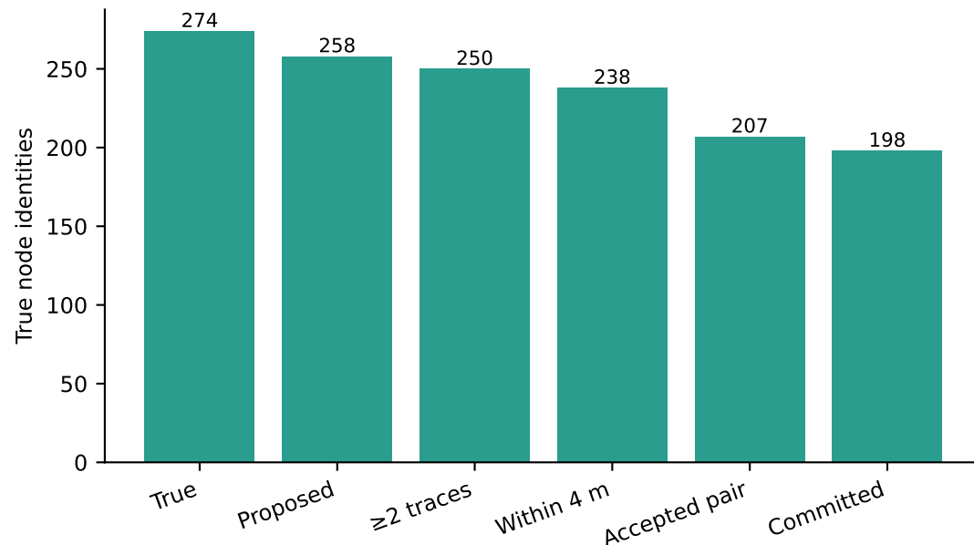
Why traversed edges are still lost
