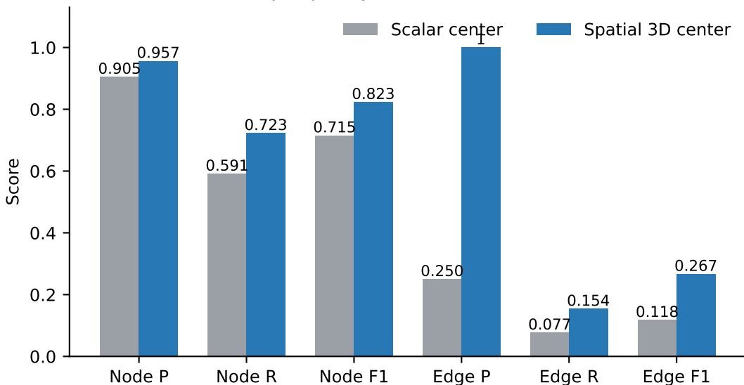
Graph quality on unseen C07-C08
