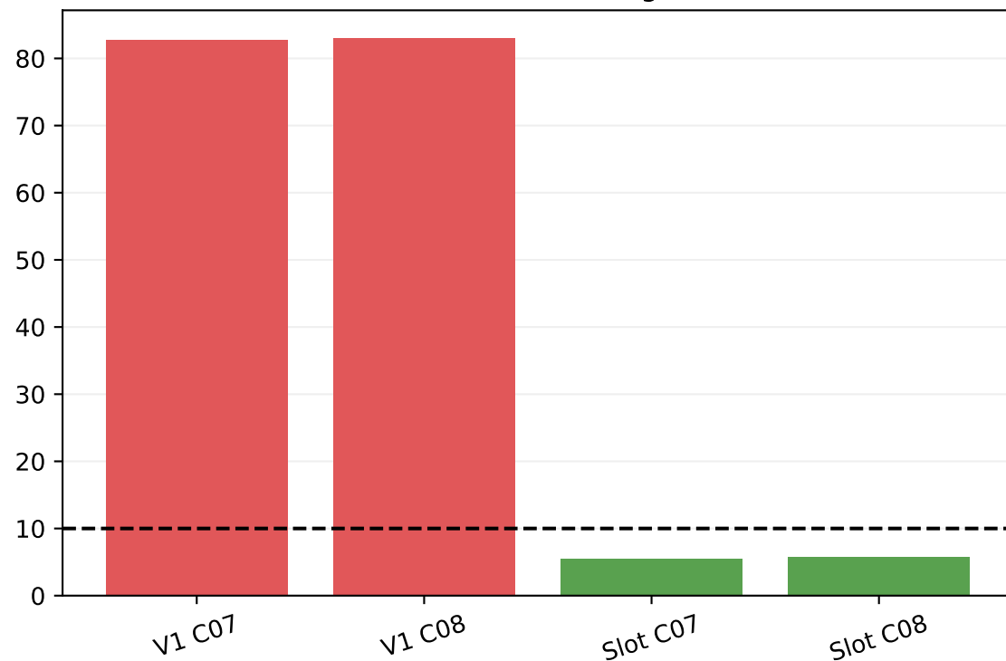
C Exact-bin average precision
