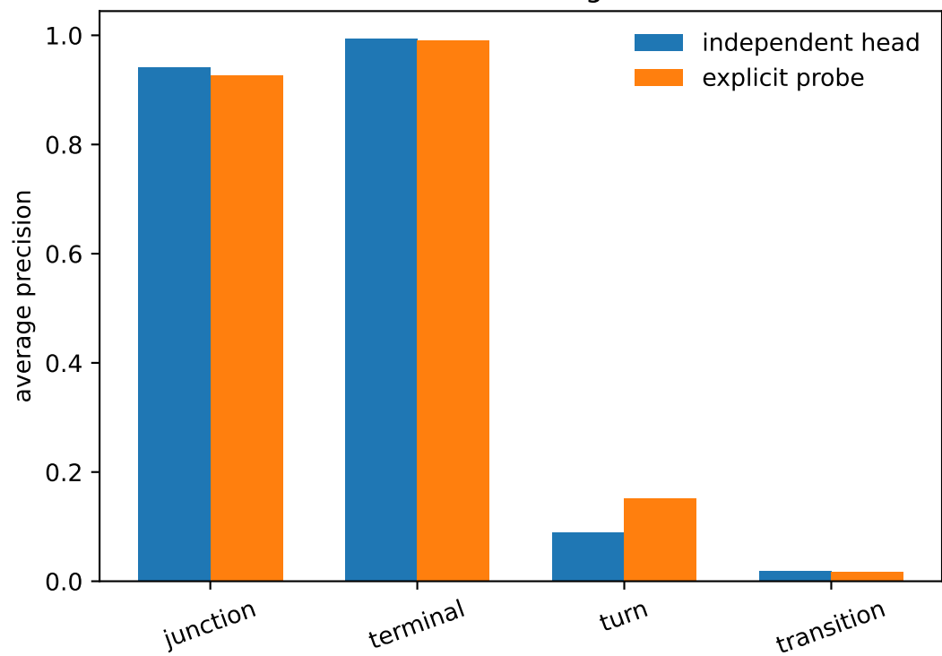
Rare-event ranking on C08
