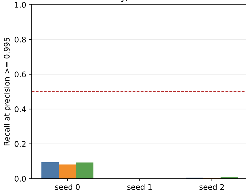
B Safety/recall contract
