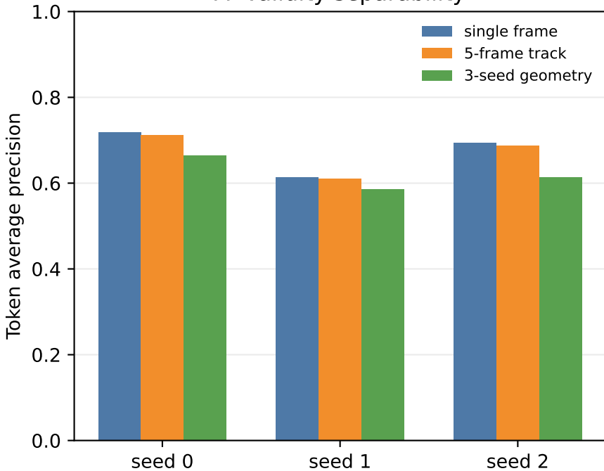
A Validity separability
