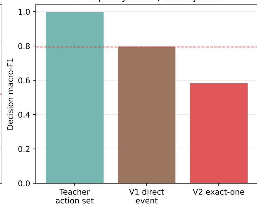
C Capacity exists; validity fails
