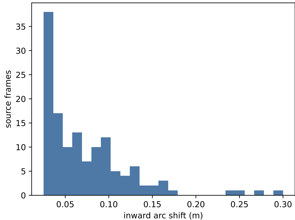
Only invalid endpoint poses move
