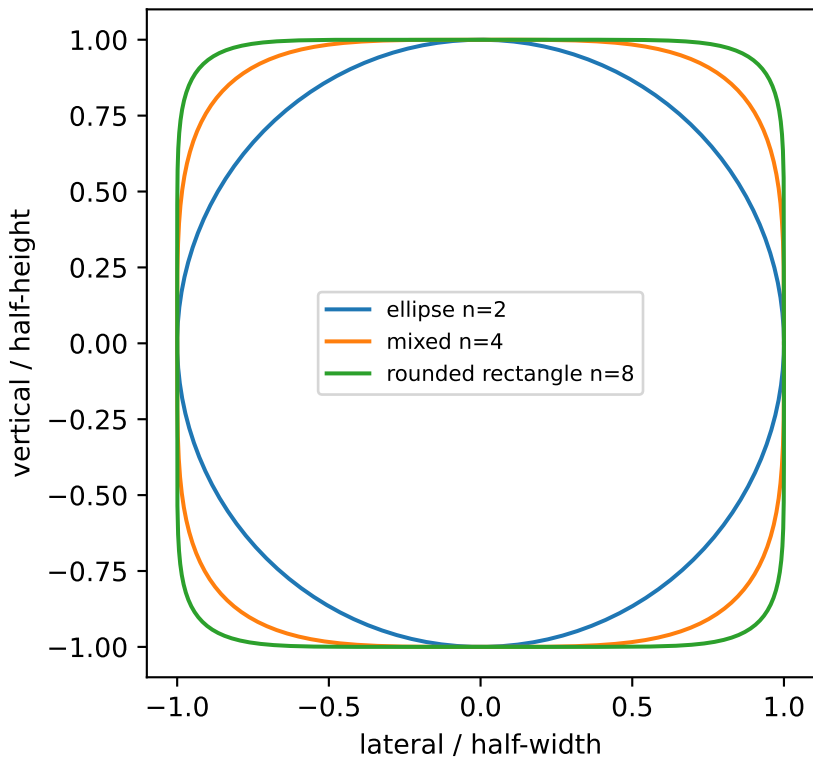
One continuous cross-section family
