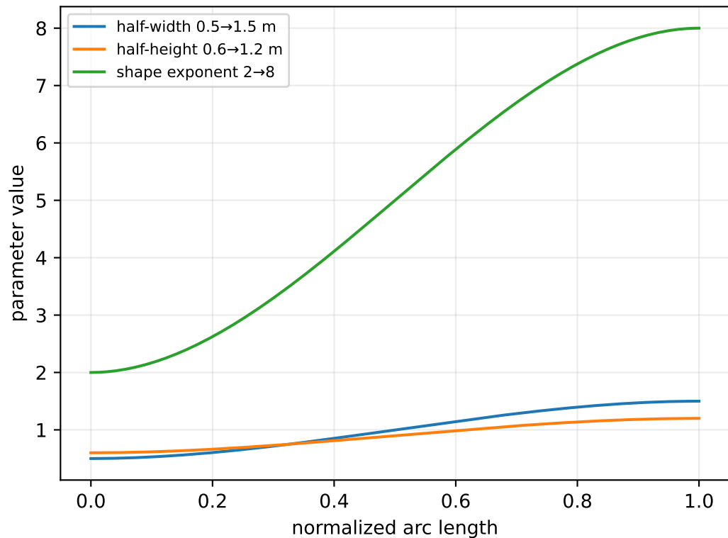
C1 taper and shape transition
