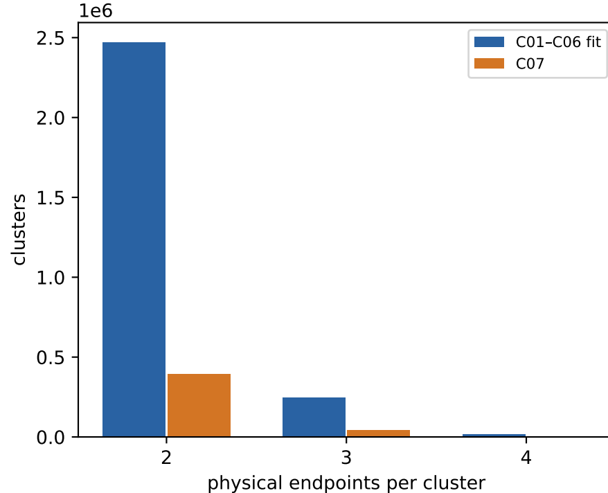
Primitive Connection Hypergraph Teacher feasibility (fit + C07 only)
