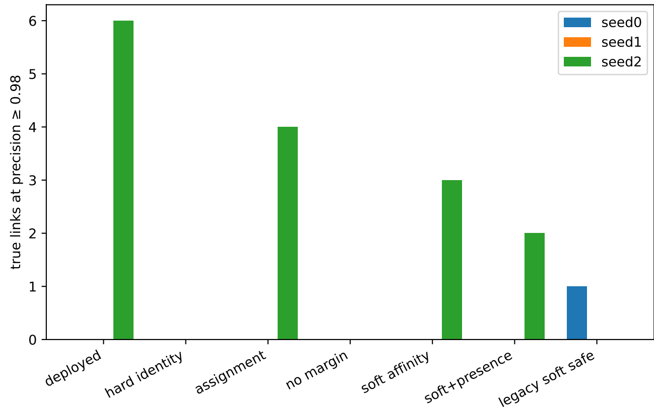
Frozen local-slot failure attribution on C07
