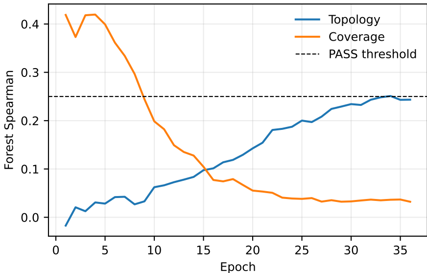
Semantic bottleneck validation trajectory
