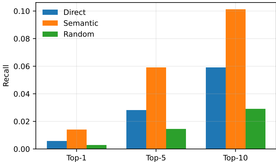
Forest cross-position retrieval
