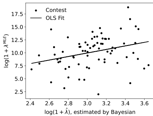
Figure 8 Robustness Check (2nd–3rd Pair): \lambda^{MLE} vs. Bayesian Estimate \hat{\lambda}
