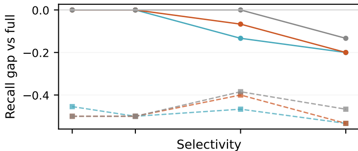
GIST1M high-acc
