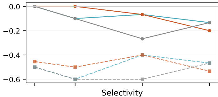
GIST1M zk-opt
