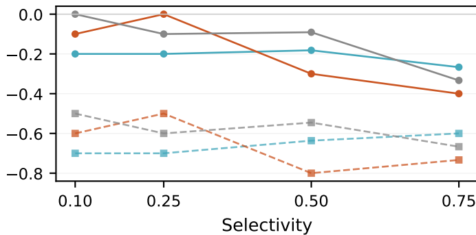
GIST1M high-acc
