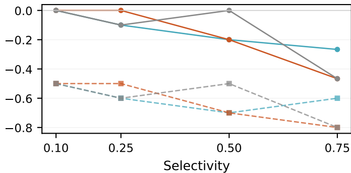
GIST1M zk-opt
